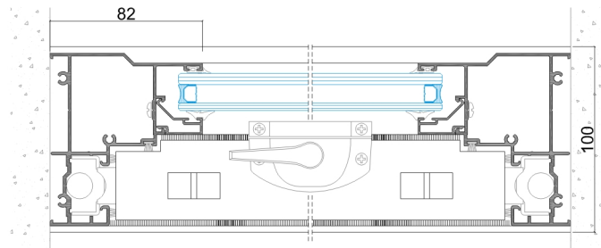
Corte pela folha superior Detail of upper leaf | Coupe de la vantail supérieure
