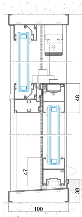
Corte vertical Vertical section | Coupe verticale
