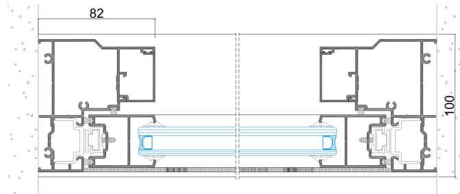
Corte pela folha inferior Detail of lower leaf | Coupe de la vantail inférieure
